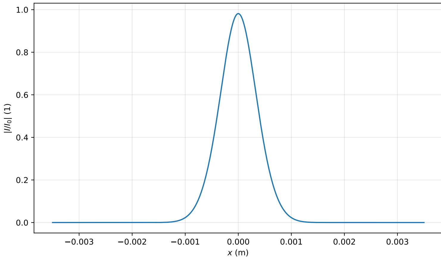
Intensity profile I(x, y = 0, z = 0.716m)/I_0 , P_{in}=0.3P_{cr} , artificial time
